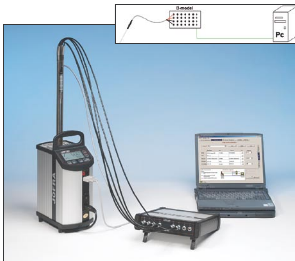
Picture 2: ASM-803 B performing its own measurements in a JOFRA ITC-320 A including an STS reference sensor in channel one all controlled by JOFRACAL.
