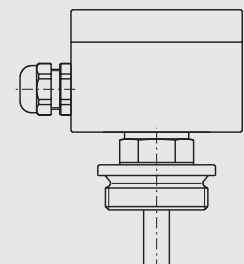
Mounting thread and connection housing
